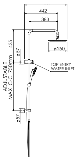
Brushed Gold TRCBG
