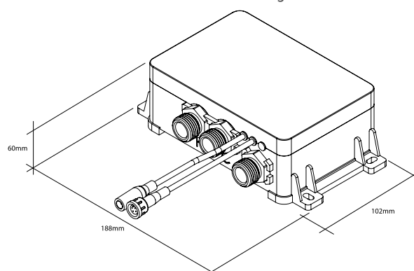
Digital mixer
