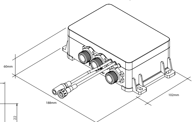
Digital mixer
