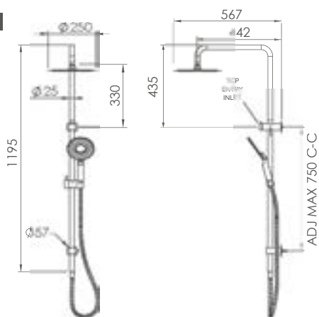
H2RSCC TOP ENTRY INLET
