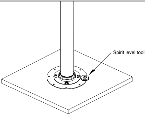
6. Using the supplied spirit level, ensure base mount and mixer are level. If the mixer is twisted or uneven the o-ring seal in the base mounts may dislodge and leak.
