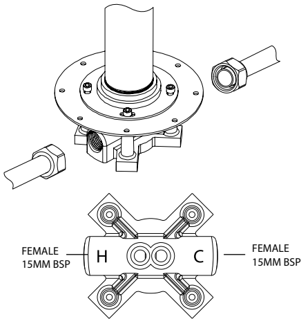
8. Connect the hot and cold water source to the mixer location. Make sure to purge the pipe before connecting to the mixer. Test watertightness.
