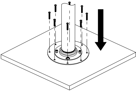
7. Using the 8 supplied wood screws, fix the bath filler into the wood floor.
